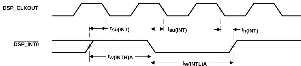
Figure 6–12. Interrupt Timing
